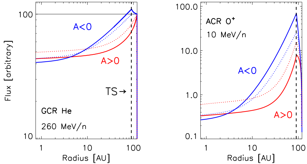
Fig. 3. 2D simulation of GCR He transport from the heliopause to 1 AU and ACR oxygen from the termination shock to 1 AU for qA > 0 and qA < 0 solar minimum periods with K_{\parallel} = 5 \times 10^{22} \text{ cm}^2/\text{s} and K_{\perp} / K_{\parallel} = .02 . The solid lines are for \lambda = 0 and the dashed lines immediately adjacent to these curves are for a heliolatitude of 30^\circ .
