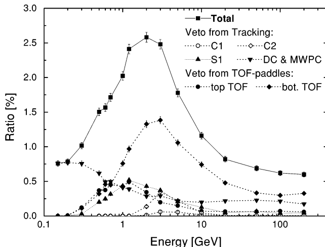
FIG. 13.—Percentage of tracks which fail both the preselection and the final cuts for Z = 1 particles because of \delta -electrons. The solid squares show the overall value.
